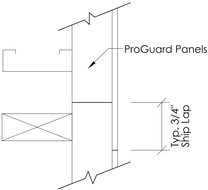
Plan View of Section
