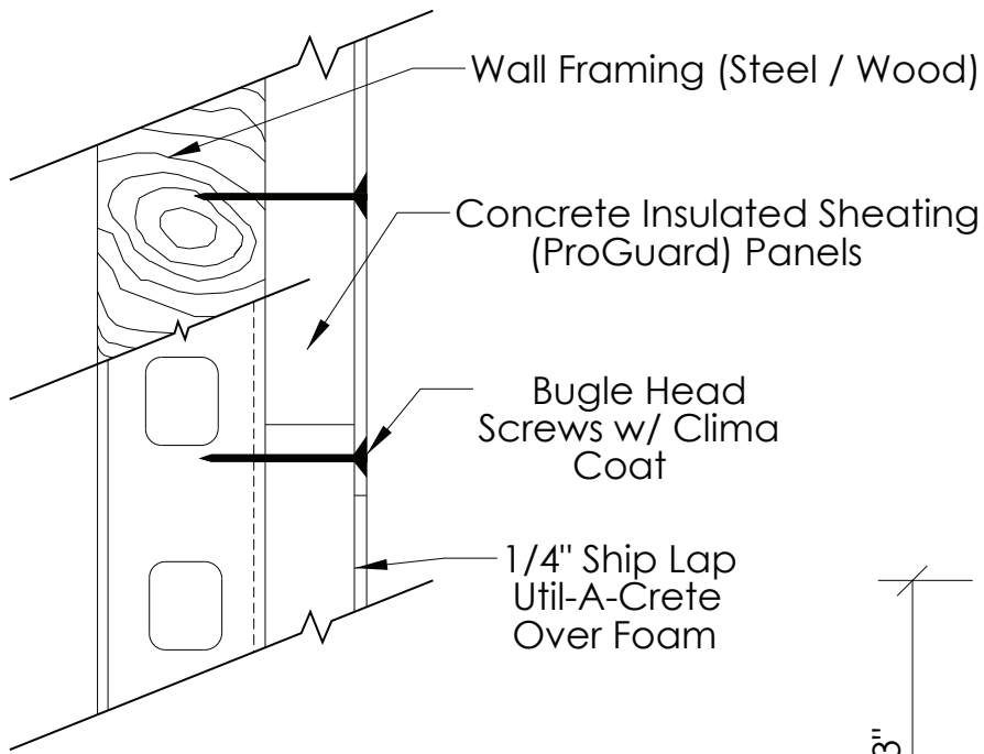
Section View of Ship Lap
