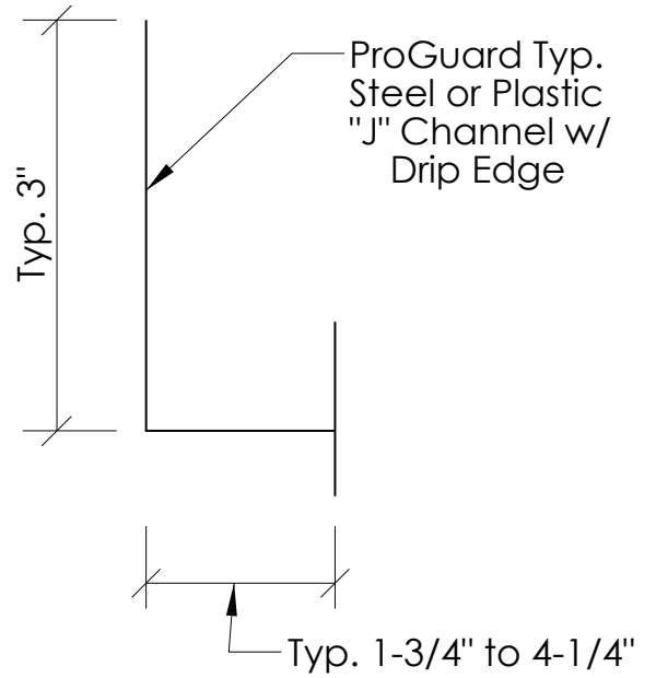
"J" Channel Detail
